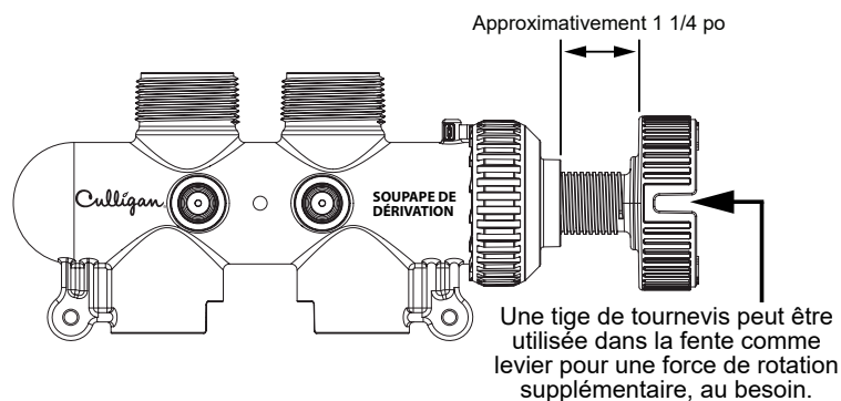
Figure 2. Vanne de service
